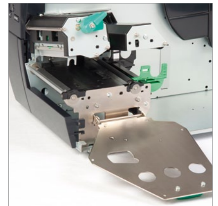
Wide opening printhead block
